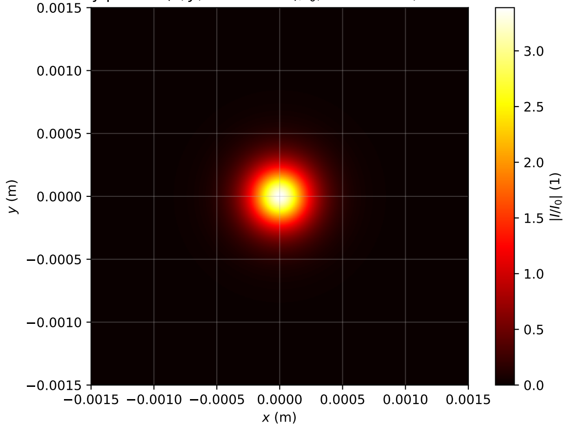
Intensity profile I(x, y, z = 3.981m)/I_0 , Pin=1.0Pcr, artificial time
